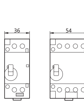
BCH8 manual control contactor 32/40/63A
